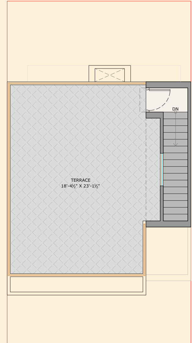
TERRACE PLAN
