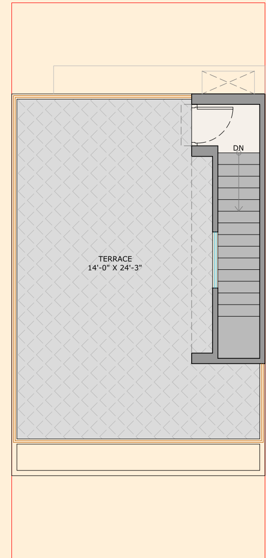
TERRACE PLAN
